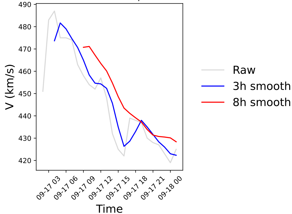
OMNI Solar Wind Speed
